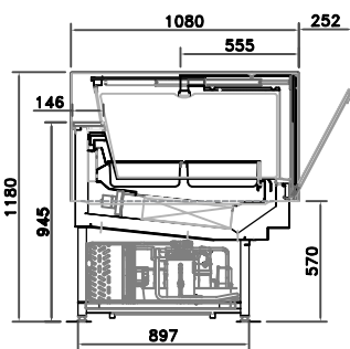
WITHOUT PANELS
