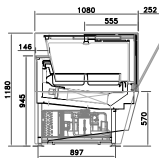
WITH PANELS
